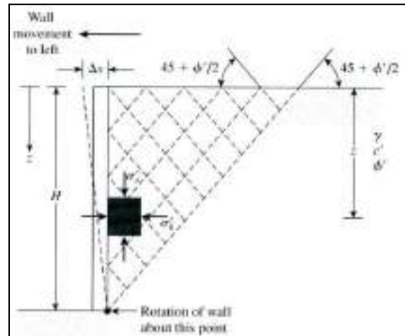
Figure 4.23: Rankine's active pressure (Das, 2011)
