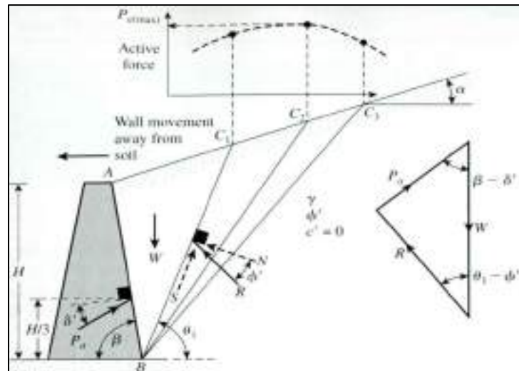
Figure 2.2: Coulomb’s active earth pressure theory
