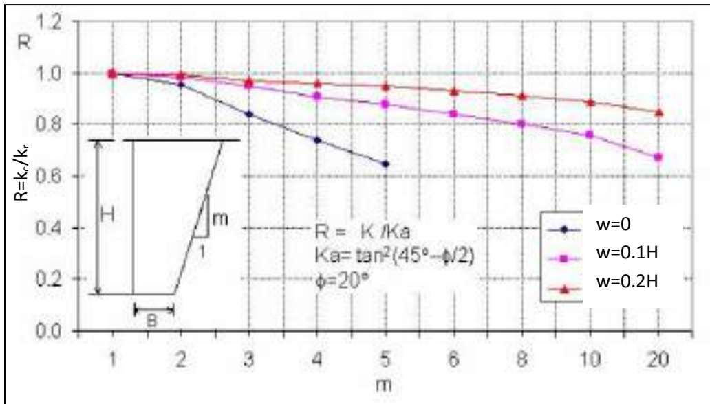
Figure 2.11: Design charts developed for an angle of internal friction equal to 20^\circ (Leshchinsky & Hu, 2003)
